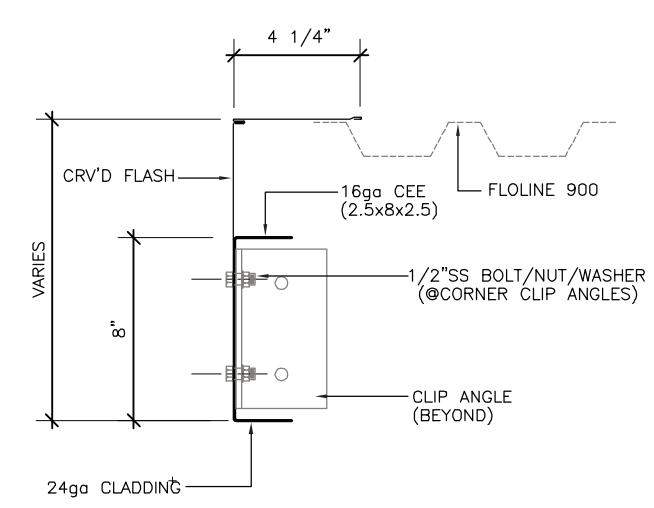
FRONT RAKE
