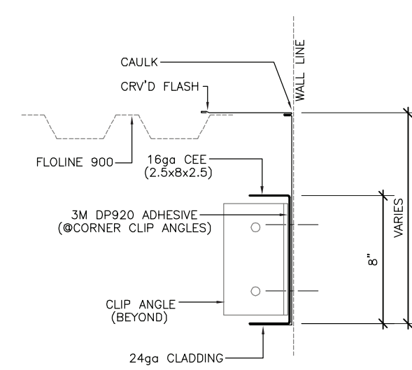
REAR RAKE
