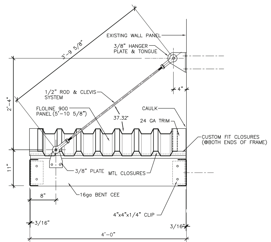
SIDE ELEVATION/SECTION
