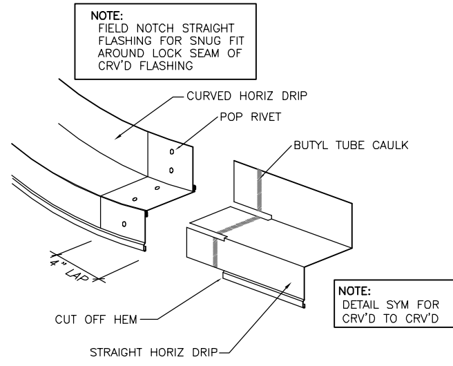
CURVED DRIP HORIZONTAL BASE
