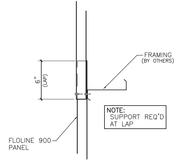
VERTICAL PANEL ENDLAP
