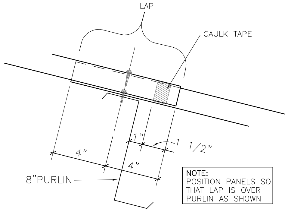
ROOF PANEL ENDLAP (CRV'D OR STRAIGHT)
