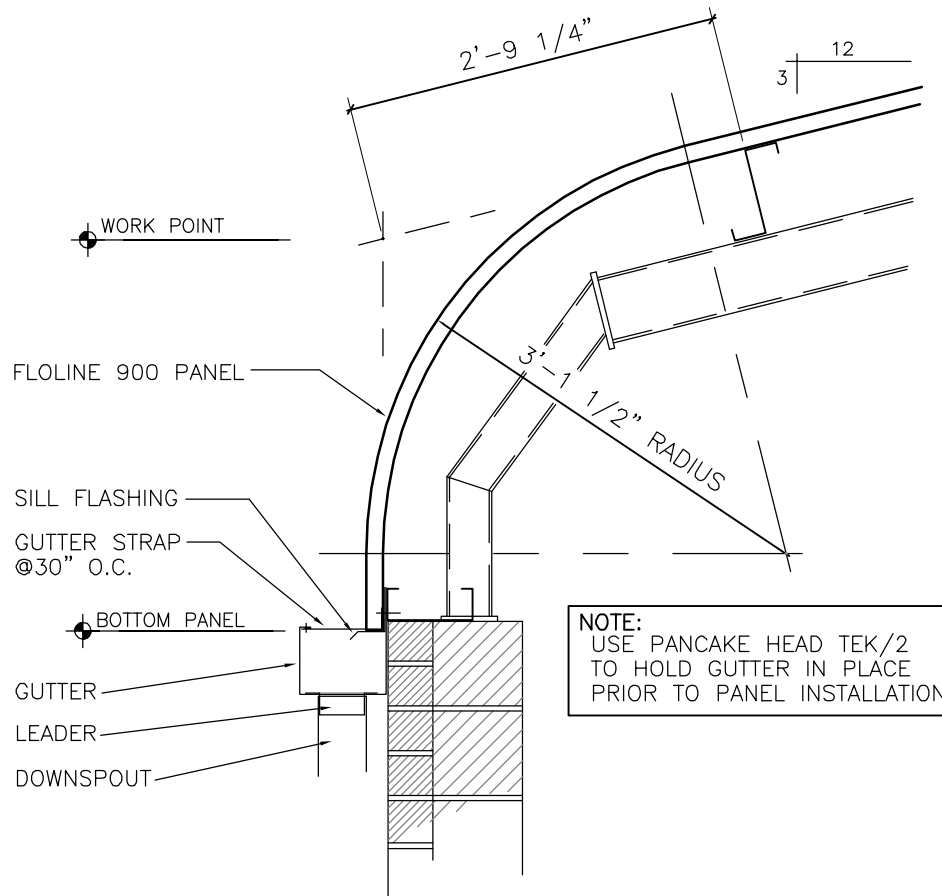
TYPICAL EXPOSED GUTTER
