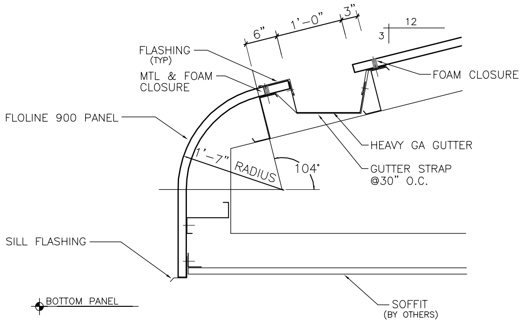
TYPICAL CONCEALED GUTTER (TYPE A)
