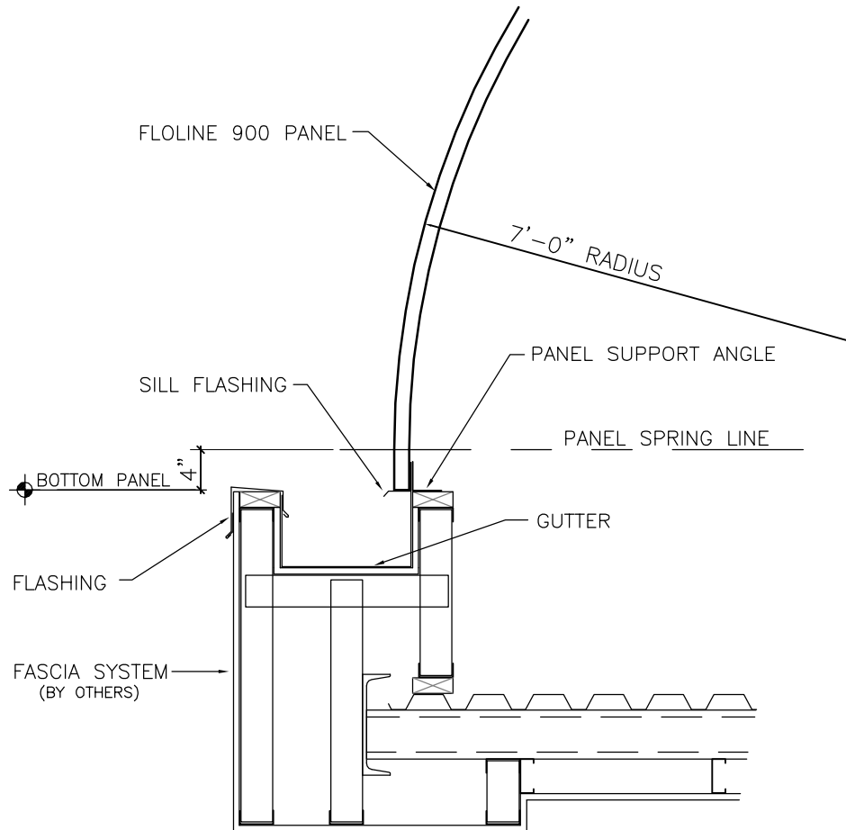
TYPICAL CONCEALED GUTTER (TYPE B)
