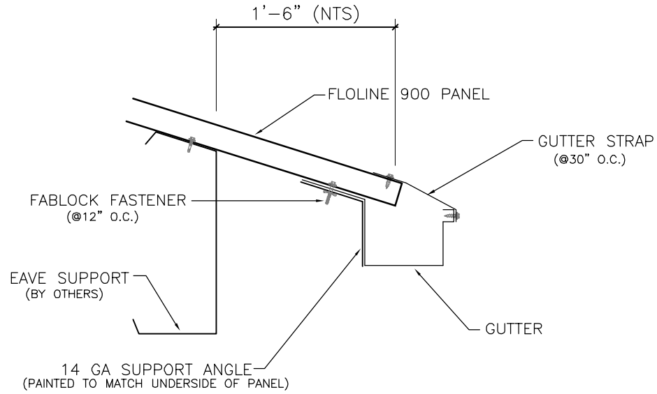
TYPICAL CANTILEVERED GUTTER
