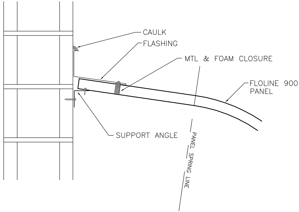
PANEL HEAD AGAINST BLOCK WALL
