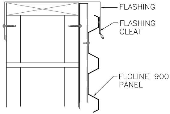
HORIZ PANEL HEAD OVER BLOCK WALL
