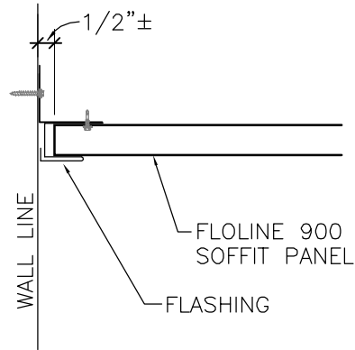
TYPICAL JAMB (SOFFIT w/o CLOSURE)
