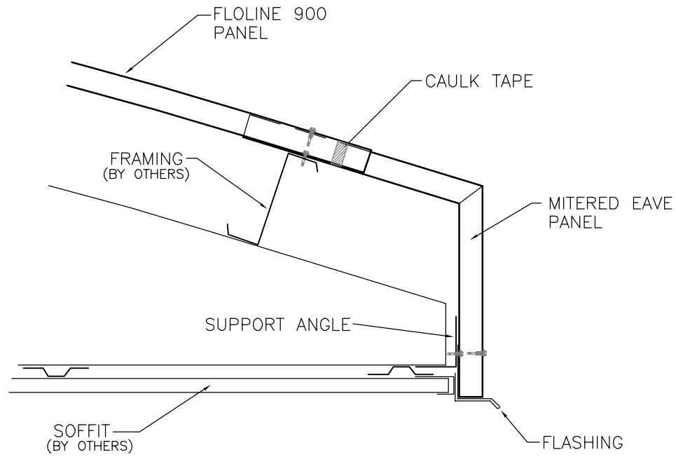
MITERED EAVE @ CURVED PANEL
