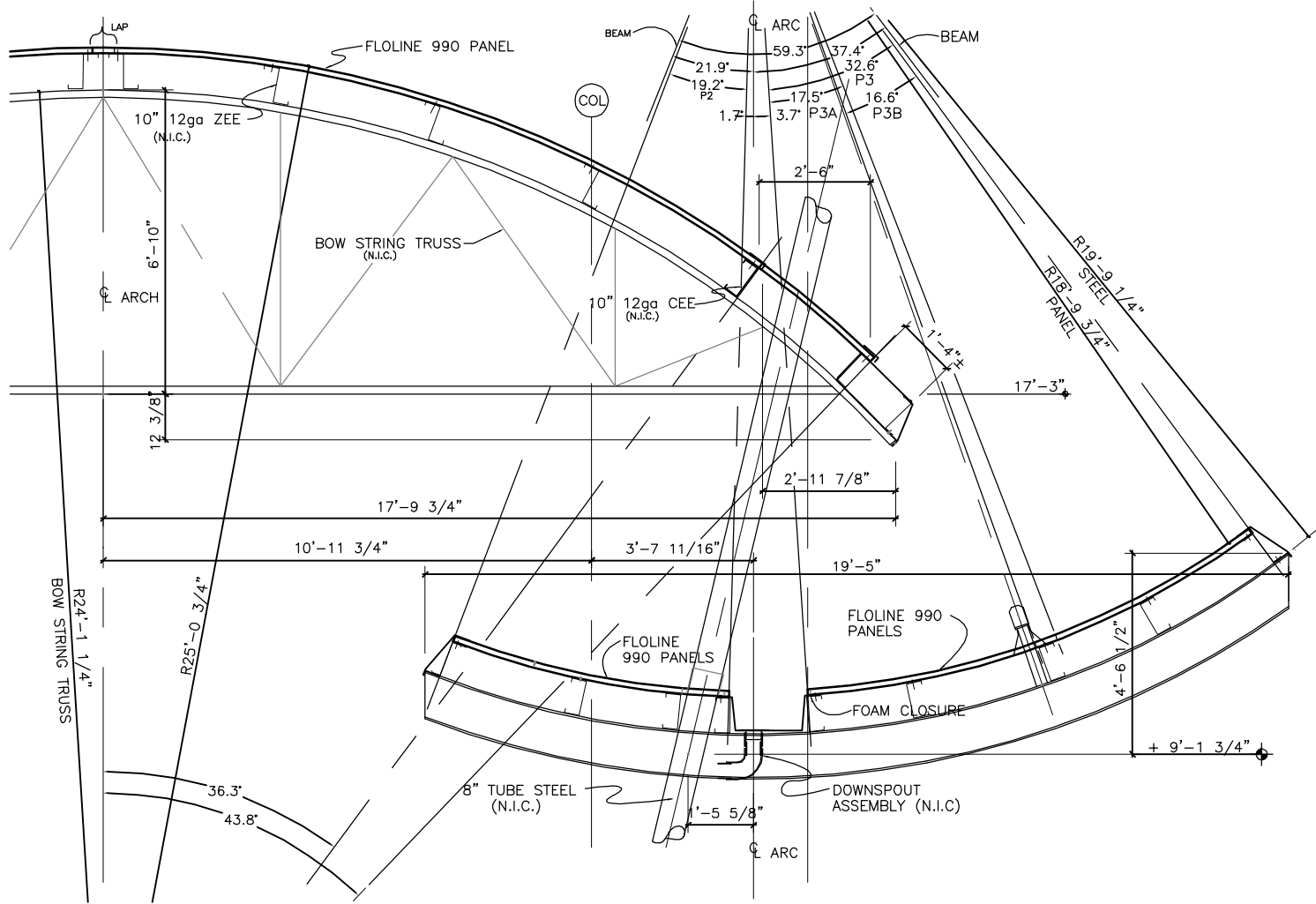
TYPICAL SECTION 78602 - PACE: SUBURBAN BUS WEB-M-05
