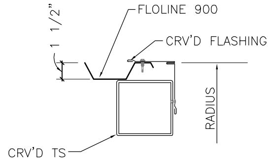
TYPICAL OUTBOARD RAKE (SINGLE LOCK CURVED)
