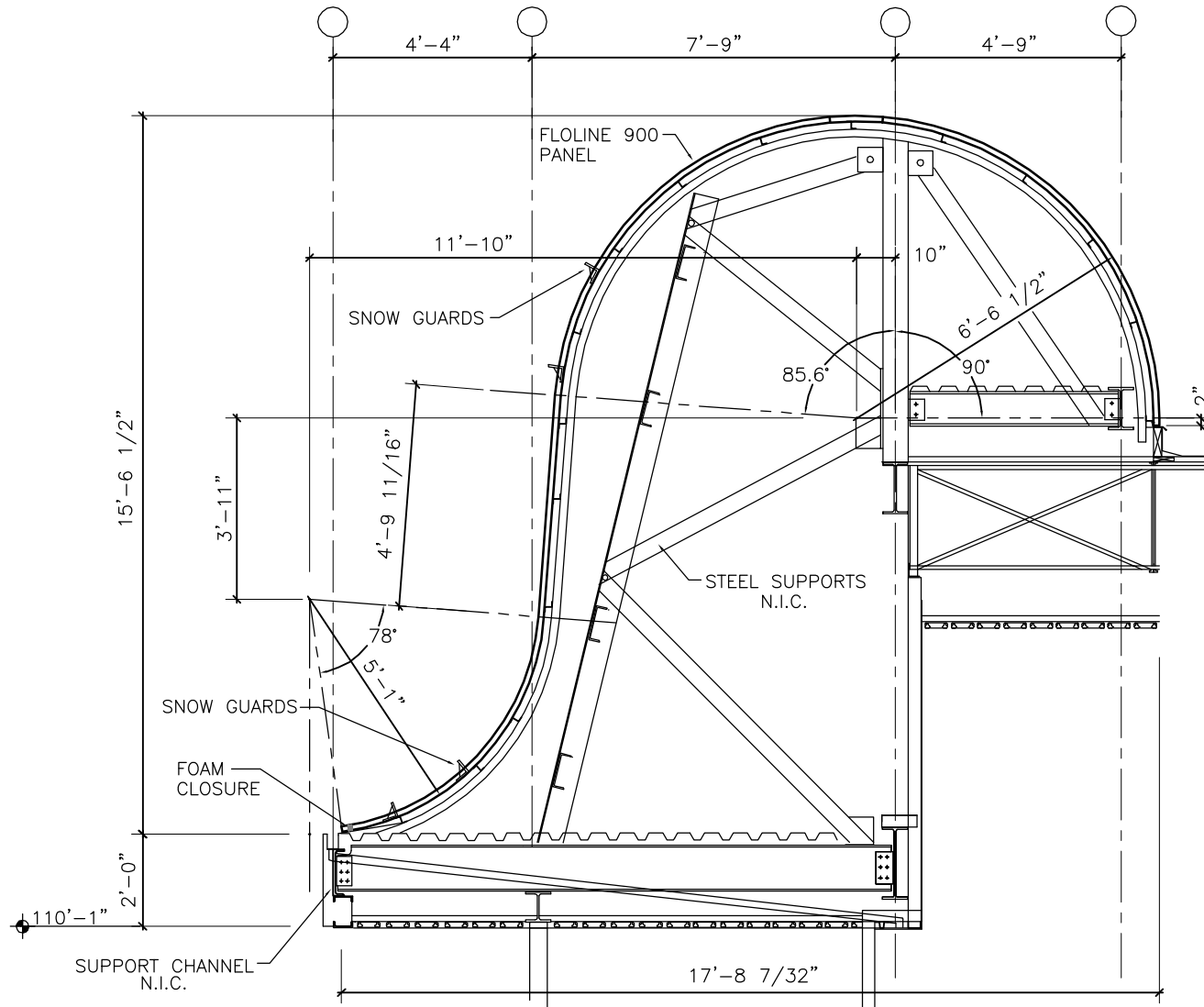
TYPICAL SECTION 98508 - SUN PUBLICATIONS WEB-0-13
