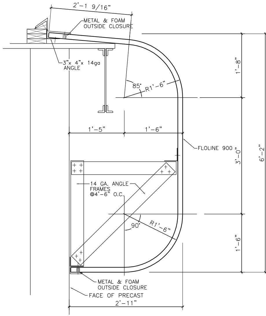
TYPICAL SECTION
